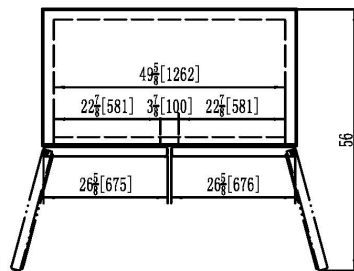
C-49FM-HC TOP VIEW
